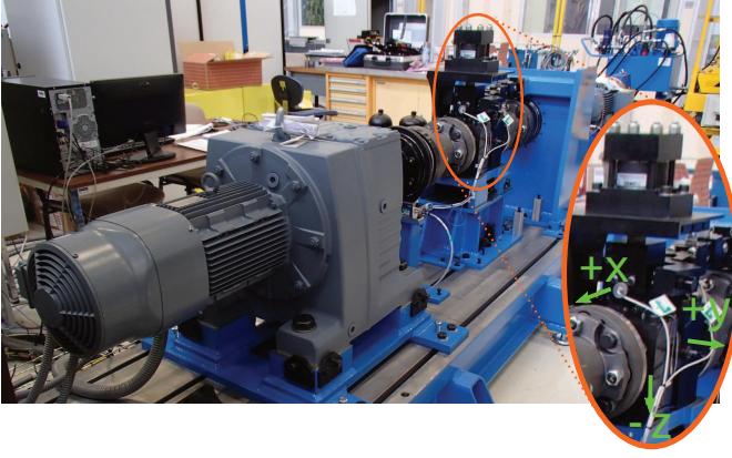
Fig. 6. A picture of the wind turbine test rig. The orange ellipsis circles the main bearing and its loading unit, while the green arrows represents the 3 wired accelerometers and their respective directions. (+x) and (+y) sensors are visible in the zoom, while (-z) sensor is hidden below the main bearing.
