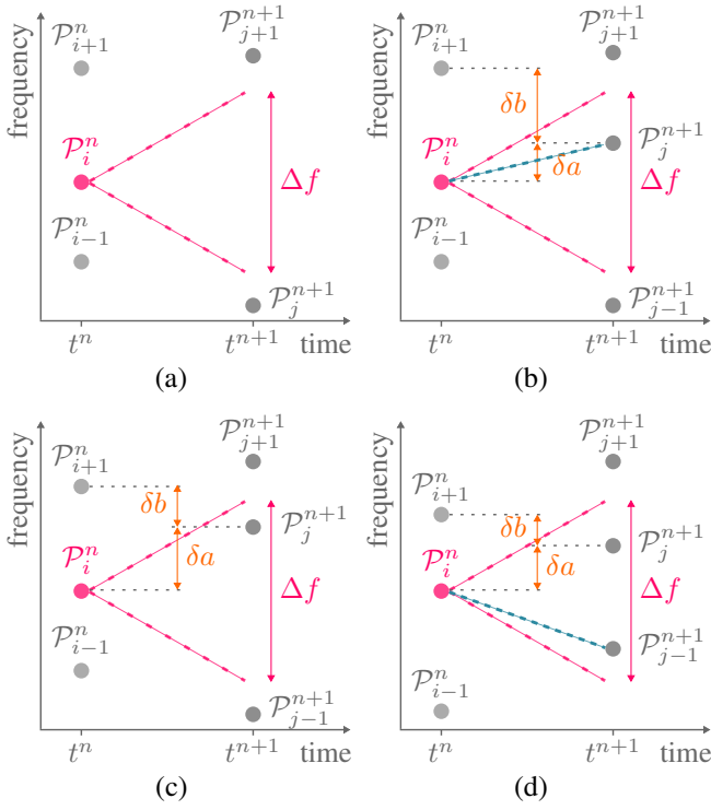
Fig. 3. Tracking of the spectral peak P_i^n (in pink): (a) there is no peak in the search interval \Delta f , the trajectory dies; (b) the only peak in the search interval verifies the backward compatibility condition \delta a < \delta b , the peak P_j^{n+1} is therefore associated to P_i^n trajectory; (c) the only peak in the search interval does not verify the backward compatibility condition, the trajectory dies; (d) the nearest peak does not verify the backward compatibility condition, the association is then done with the peak P_{j-1}^{n+1} , also present in the search interval.
