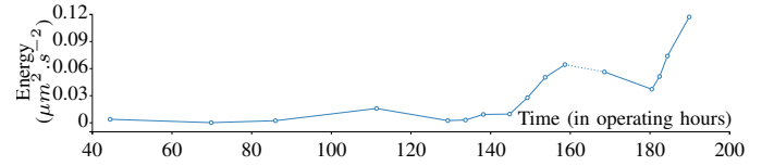
Fig. 10. After 145 operating hours, the fault is propagated: the energy of the outer ring harmonic series is also increasing.
