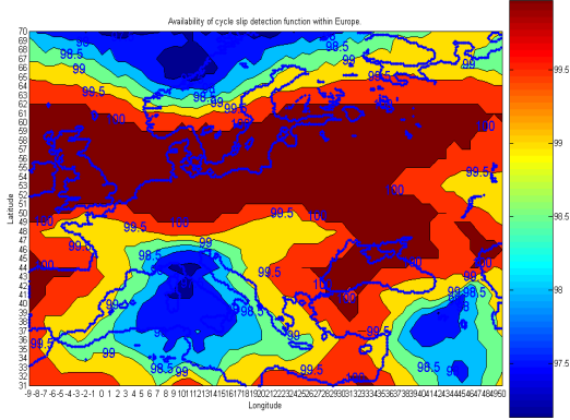
Figure 2: Availability of proposed cycle slip detection algorithm over Europe considering GPS constellation only and normal aircraft dynamics, for APV 1 alert limits.
