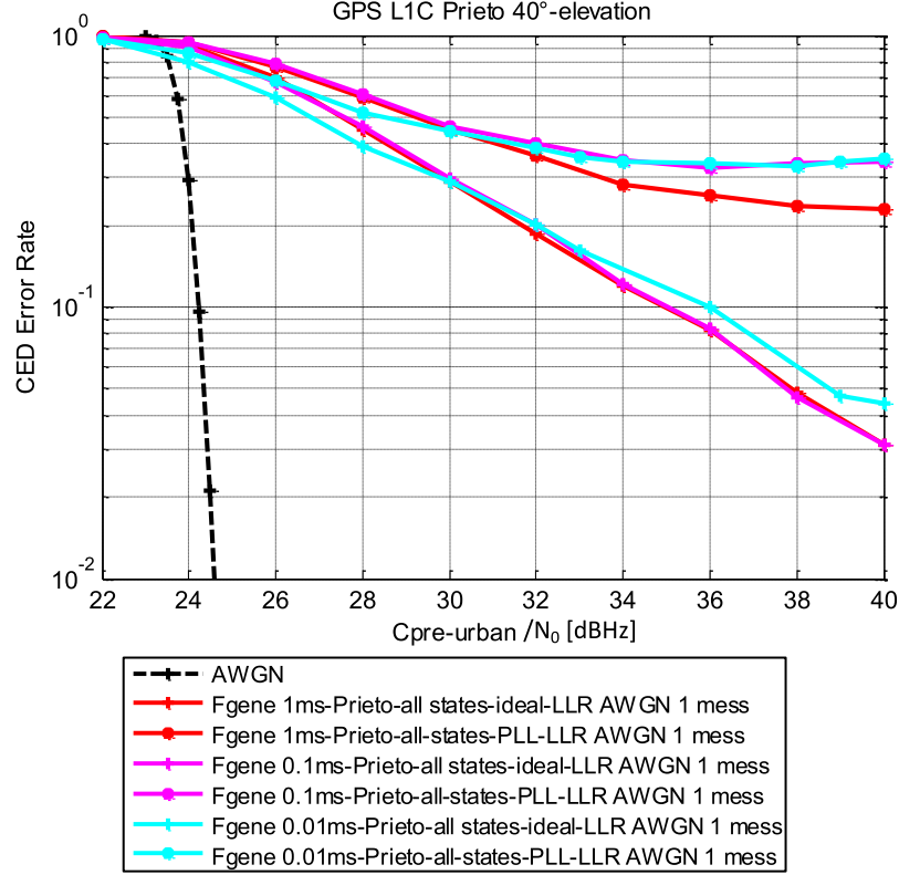
Figure 51: GPS L1C demodulation performance in the Prieto model for different propagation channel generation frequencies
