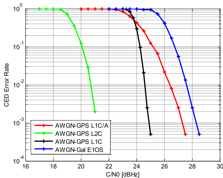
Figure 100: GNSS signals demodulation performance in the AWGN channel model with the classical methodology
