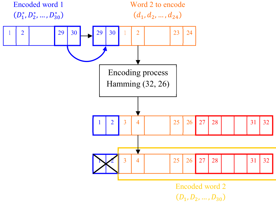
Figure 4: GPS L1 C/A channel coding description
