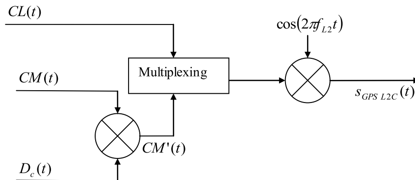
Figure 12: GPS L2C signal modulation block diagram
