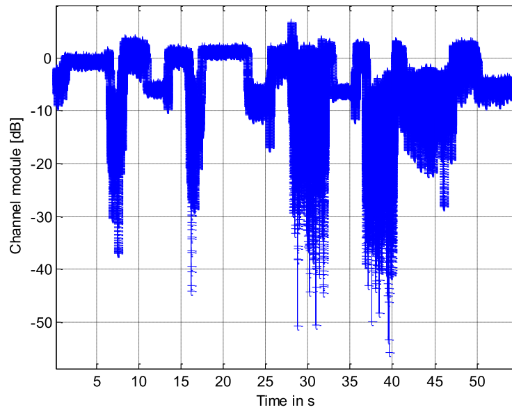
Figure 54: The received signal amplitude with the Prieto channel model
