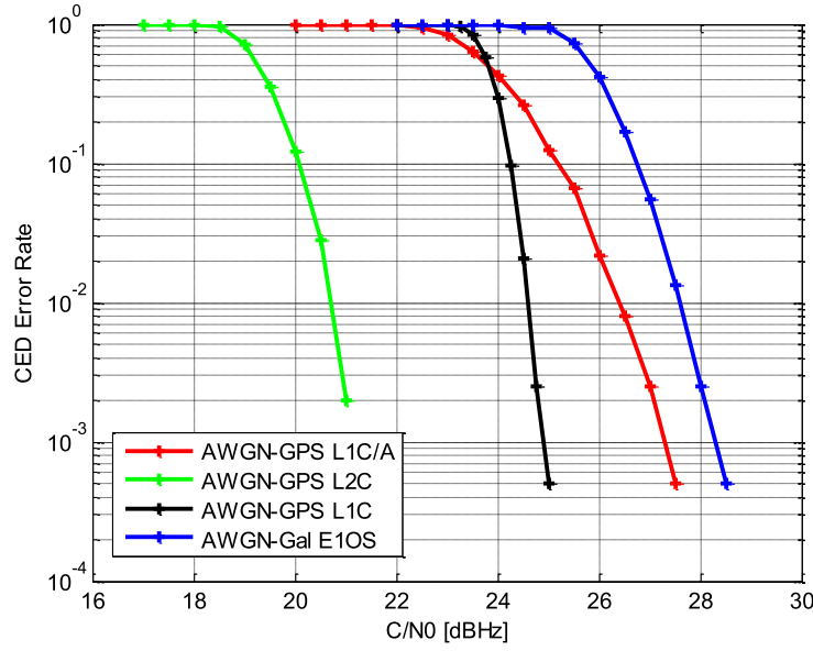
Figure 52: GNSS signals demodulation performance in the AWGN channel model with the classical methodology
