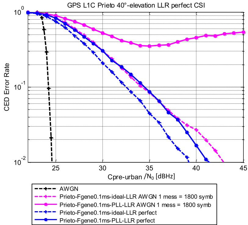
Figure 80: GPS L1C demodulation performance obtained with LLR_{perfect\ CSI} in the Prieto channel model
