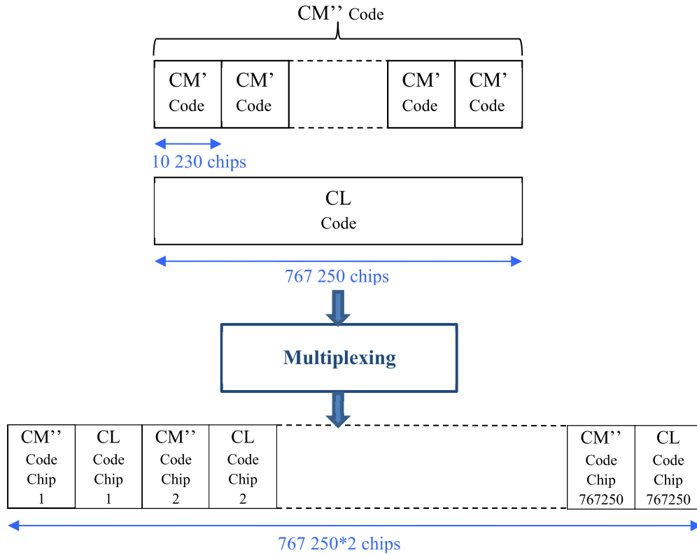
Figure 11 : Multiplexing process for CM and CL PRN codes
