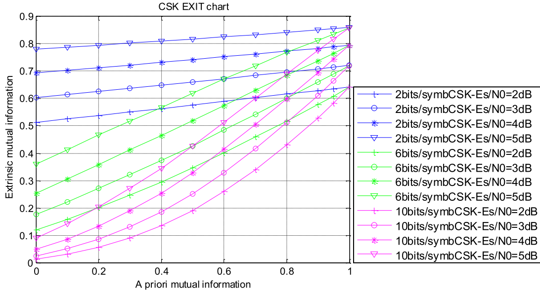
Figure 93: CSK EXIT charts for different numbers of bits per CSK symbols
