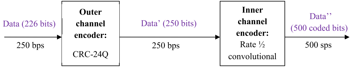
Figure 9: SBAS channel encoding description
