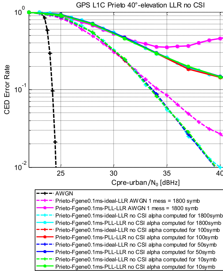
Figure 81: GPS L1C demodulation performance obtained with LLR_{no\ CSI} in the Prieto channel model
