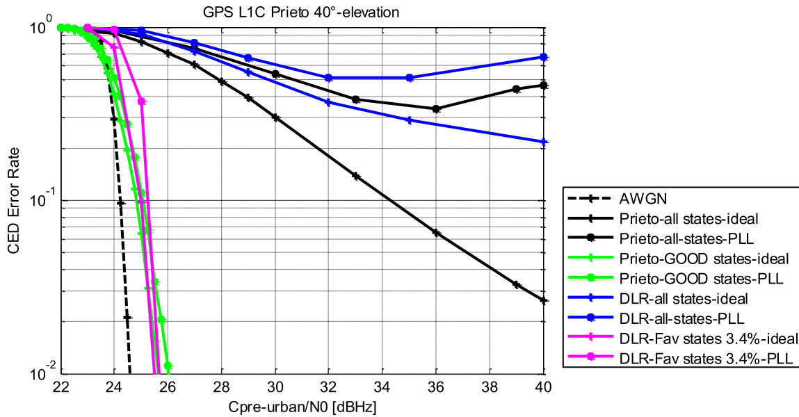
Figure 68: GPS L1C favorable states CED demodulation performance and total demodulation performance with the DLR model
