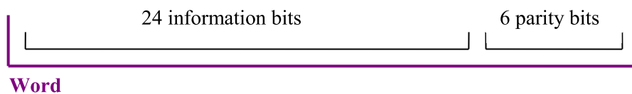
Figure 3: GPS L1 C/A navigation message word structure
