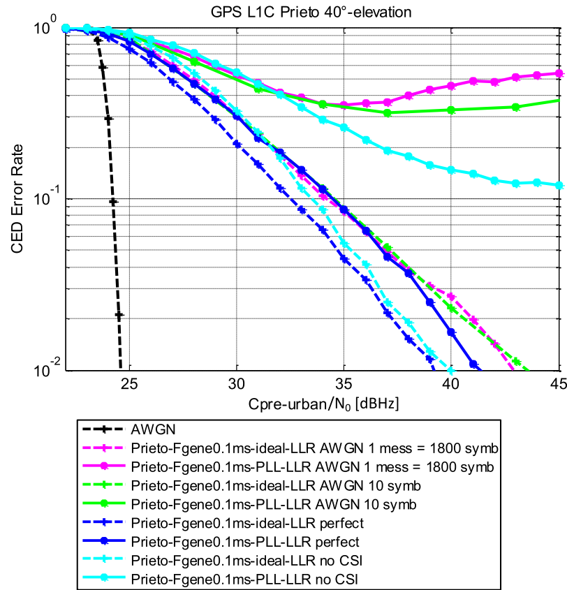
Figure 82 : GPS L1C demodulation performance obtained with advanced detection functions in the Prieto channel model
