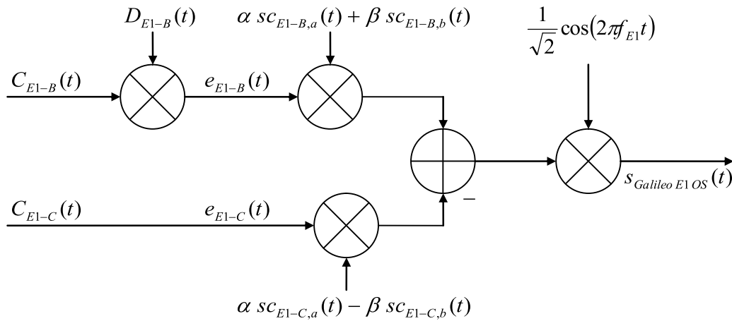
Figure 15 : Galileo E1 OS signal modulation block diagram
