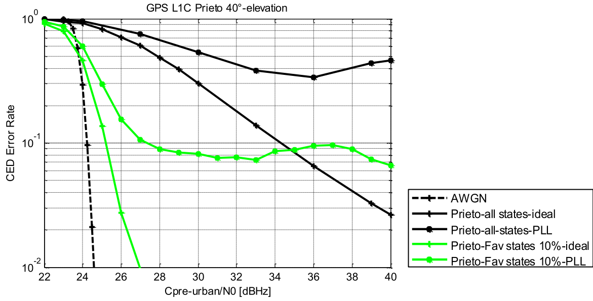
Figure 71: Favorable states subframe 3 demodulation performance and total demodulation performance with the Prieto model
