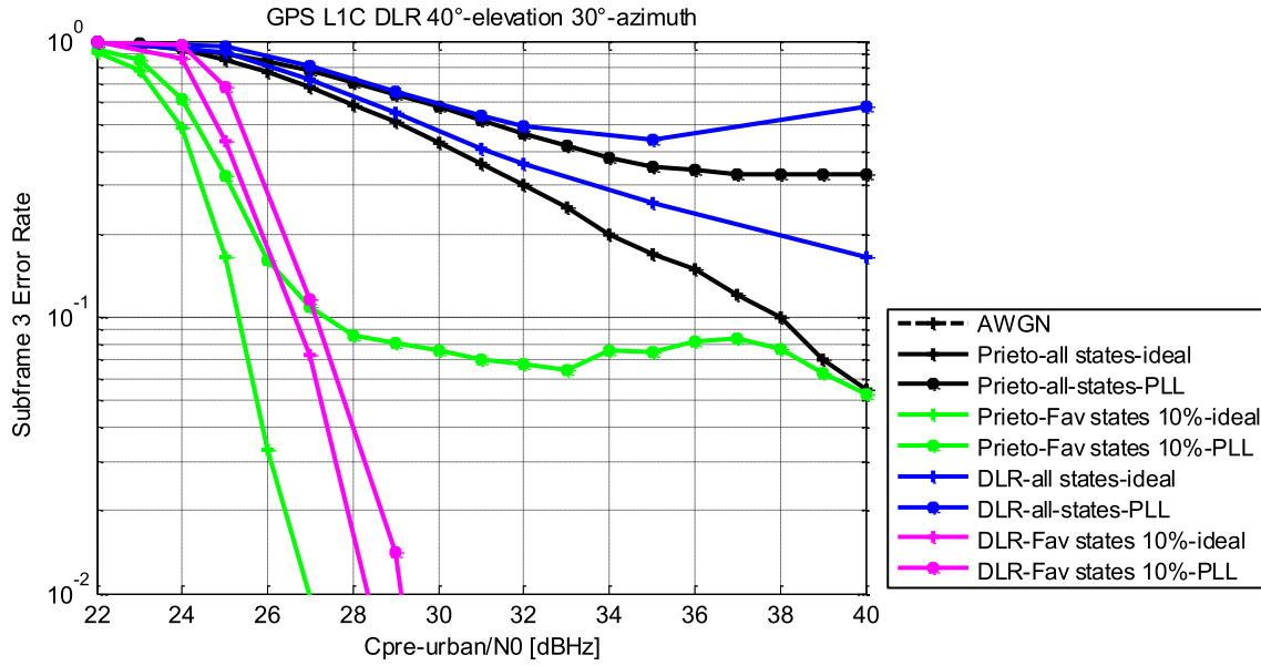
Figure 73: Favorable states subframe 3 demodulation performance and total demodulation performance with the DLR model
