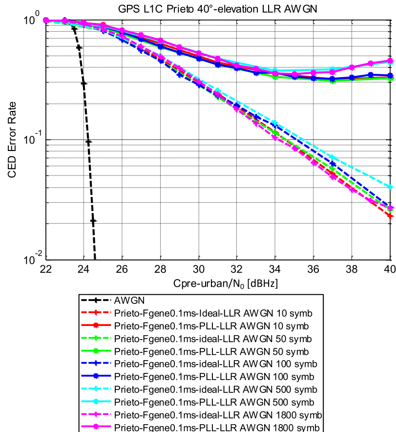
Figure 77: GPS L1C demodulation performance obtained with LLR_{AWGN} in the Prieto channel model
