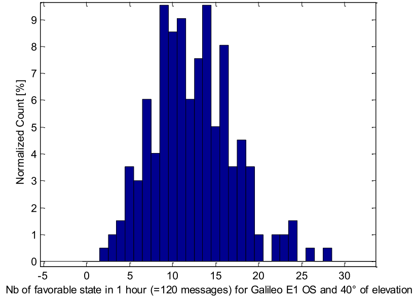
Figure 63: ‘Favorable state messages’ histogram, for Galileo E1 OS in the Prieto channel model with 40° of elevation considering the Prieto channel GOOD states as favorable reception conditions
