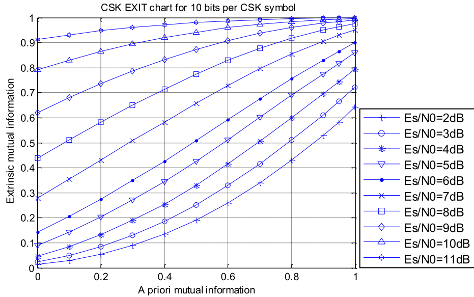
Figure 92: 10 bits CSK symbol EXIT charts for different E_s/N_0
